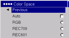
Color Space
