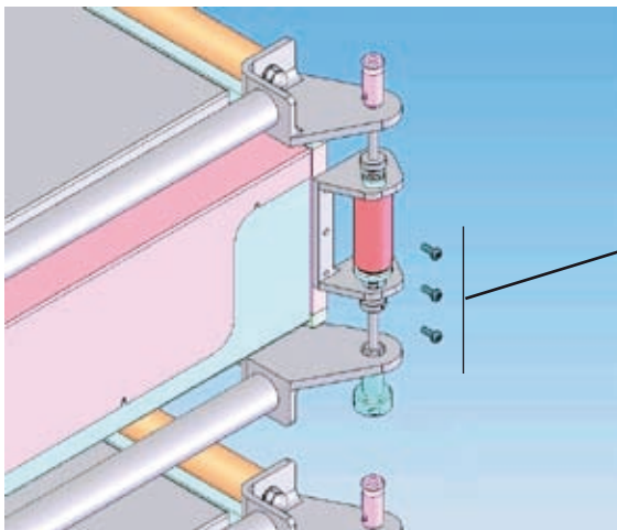
Fixing screws
