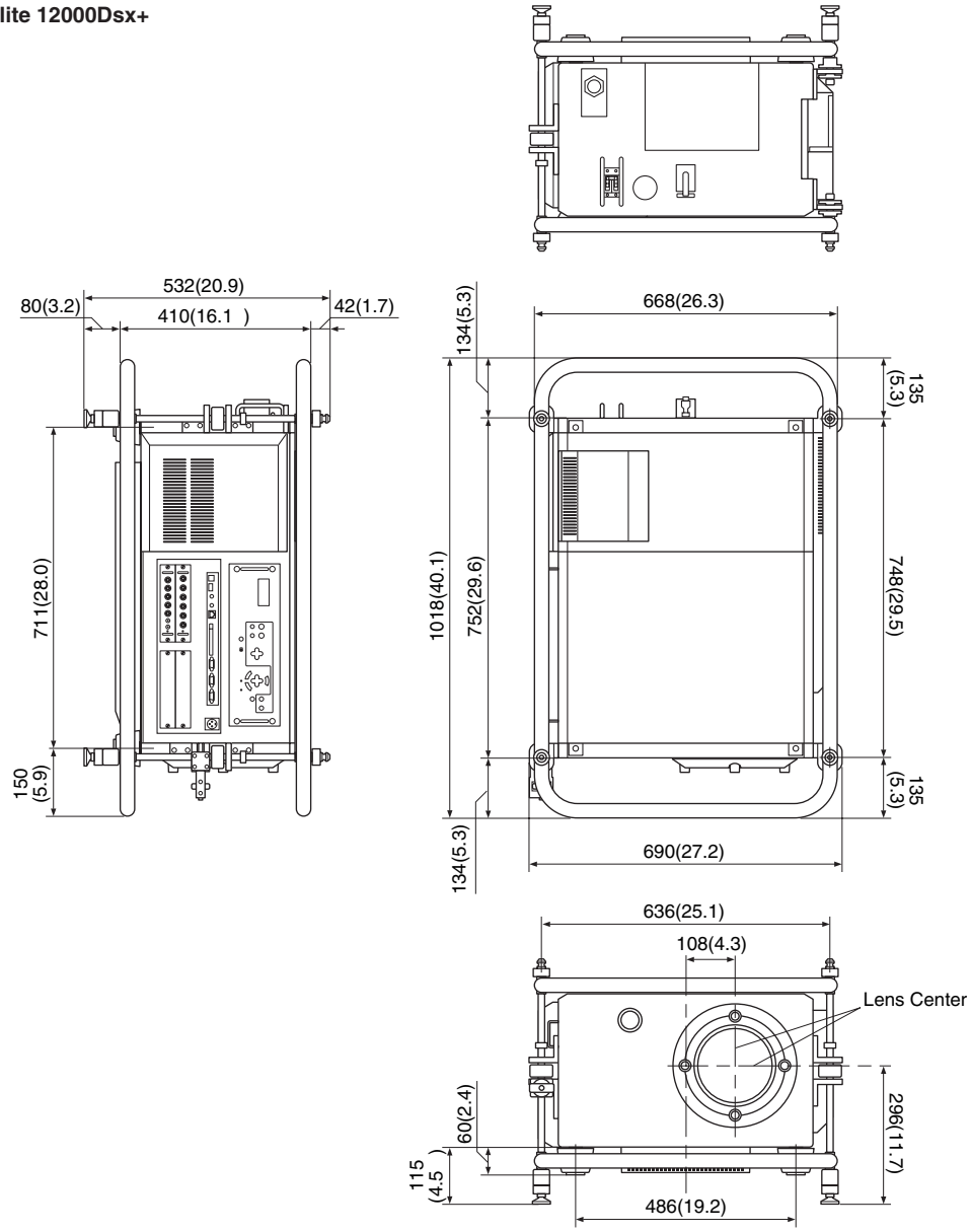
HIGHlite 12000Dsx+
