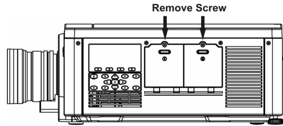
FIGURE 5-2 REPLACE LAMP
