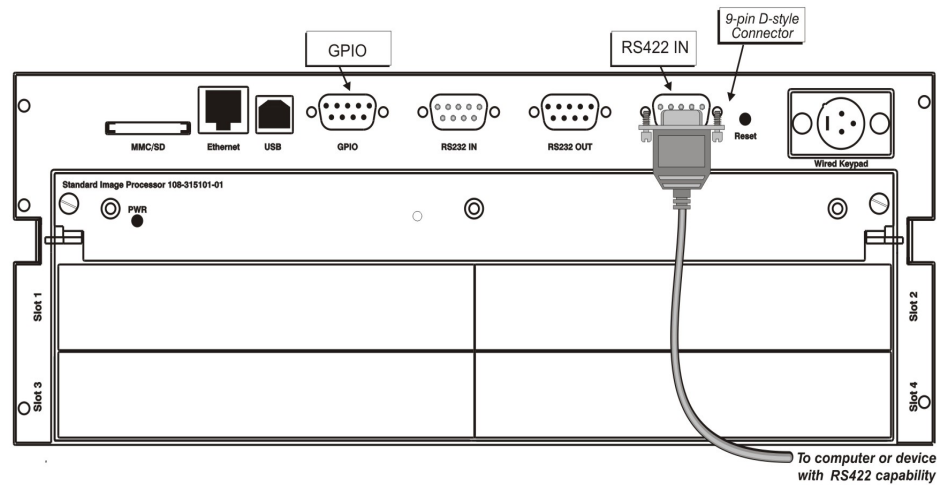
FIGURE 2-23 CONNECTING RS-422
