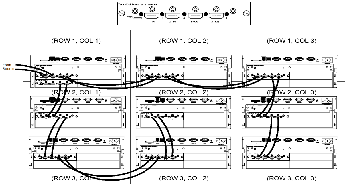
FIGURE 2-34 3X3 LOOP-THROUGH WIRING SOLUTION
