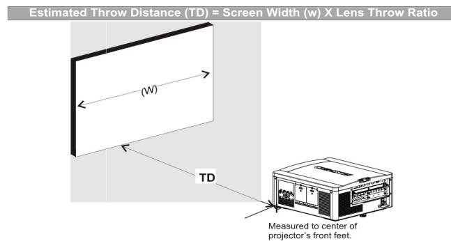
FIGURE 2-11 THROW DISTANCE
