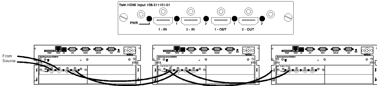
FIGURE 2-30 1x3 WIRING SOLUTION
