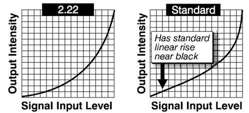
FIGURE 3-9 GAMMA CURVE
