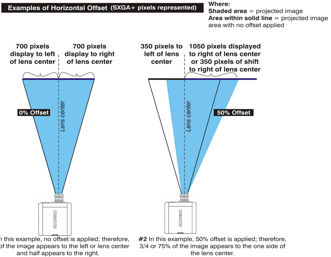
FIGURE 2-2 HORIZONTAL OFFSET EXAMPLES
