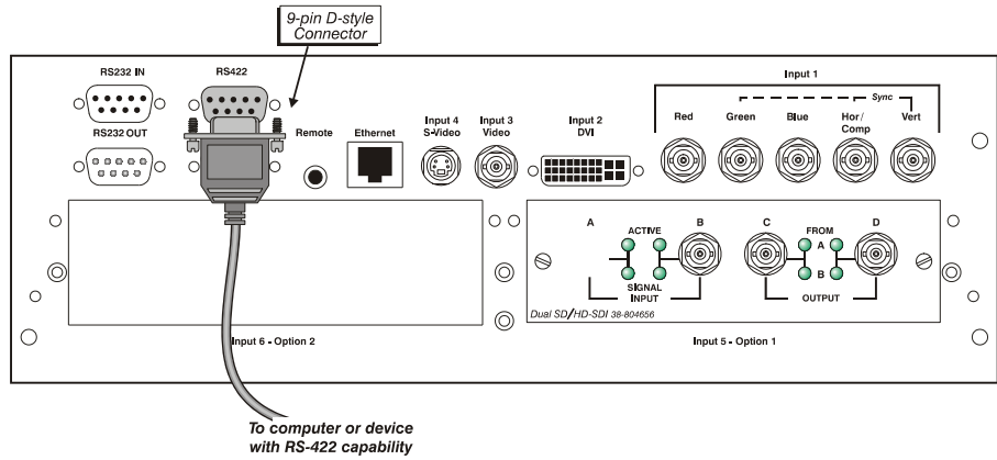
Figure 2.28. RS-422 Connection to a Computer
