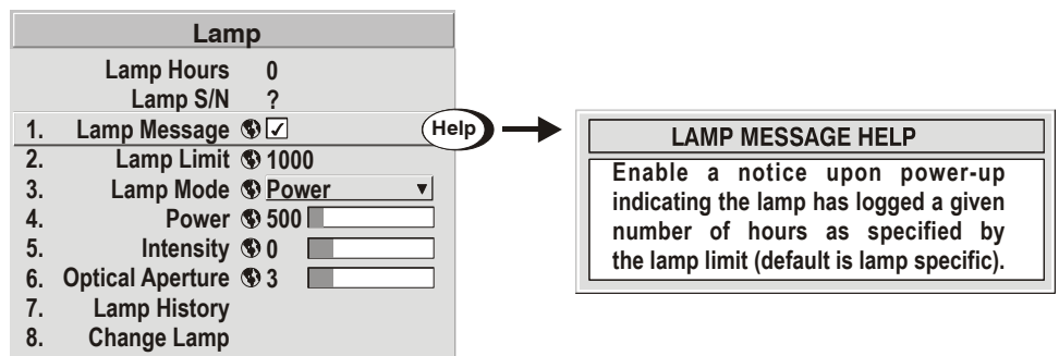
Figure 3.6. Context-sensitive Help
