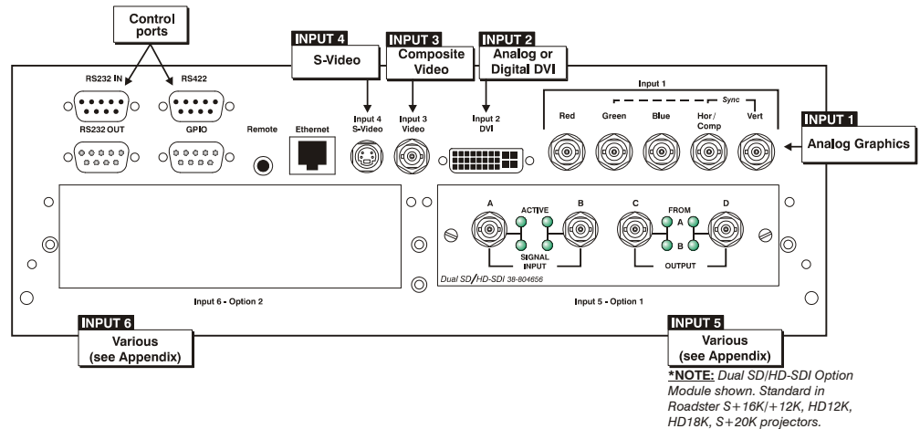
Figure 2.23. Input Panel
