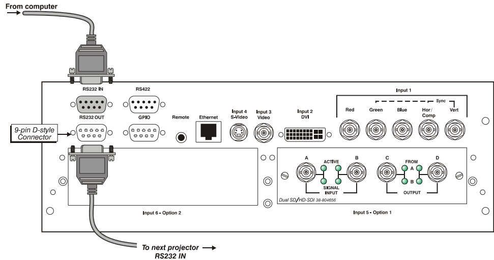
Figure 2.31. RS-232 Serial Link Loop-Through at First Projector
