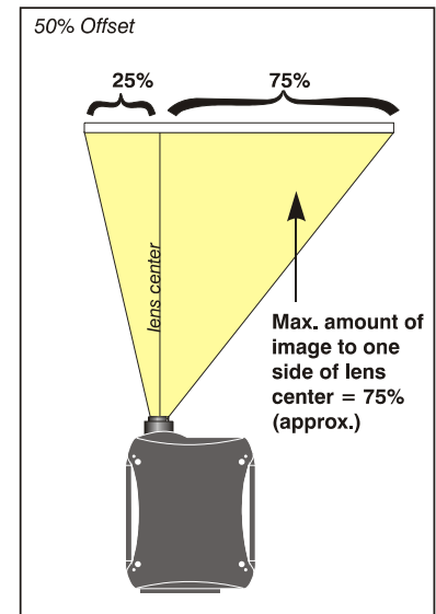
Figure 2.20. Maximum Horizontal Offsets
