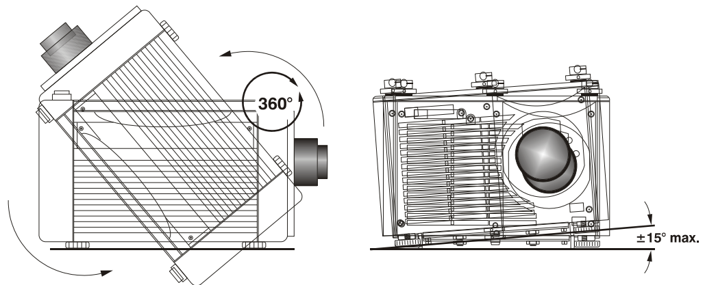
Figure 2.21. Vertical and Horizontal Tilt Ranges
