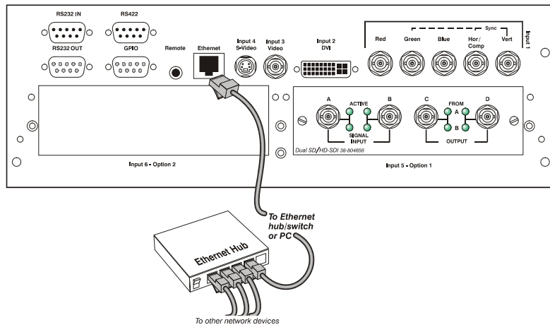
Figure 2.29. Connecting Ethernet
