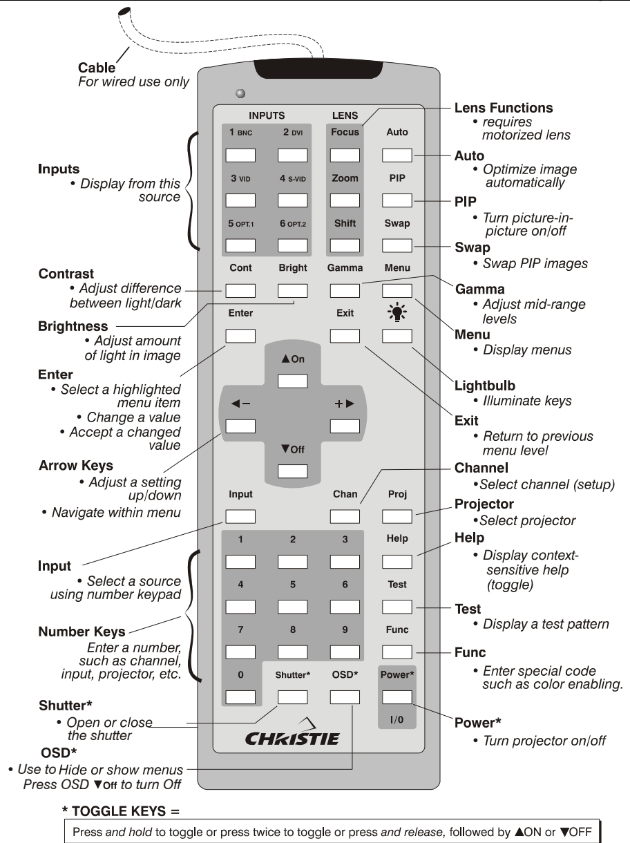
Figure 3.4. "Brick" Rental Staging – Standard IR Remote
