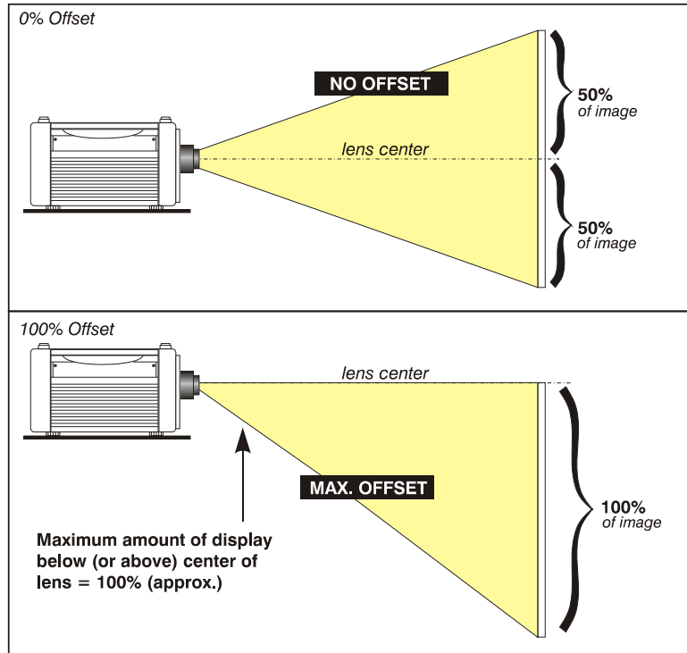
Figure 2.19. Maximum Vertical Offset
