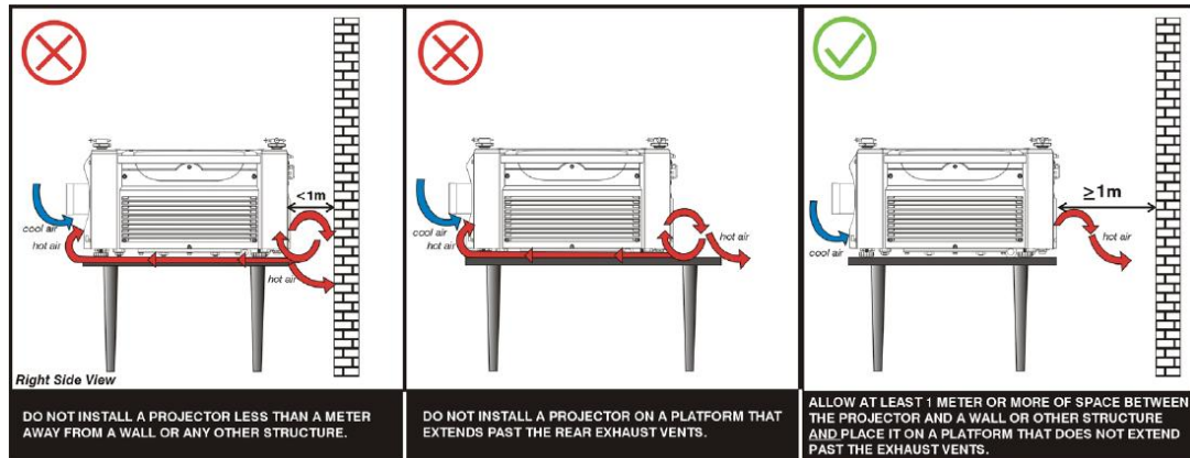
Figure 4.1. Projector positioning for proper airflow
