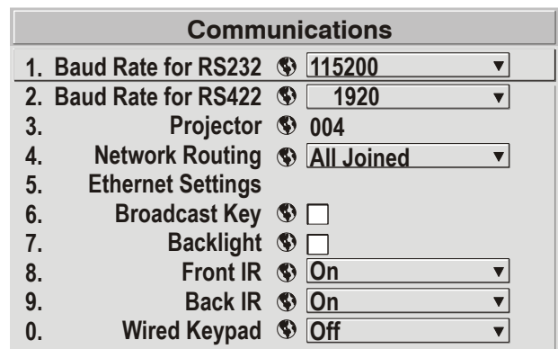
Figure 3.18. Communications
