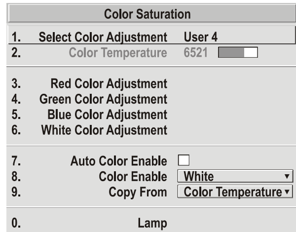
Figure 3.24. Customize Color
