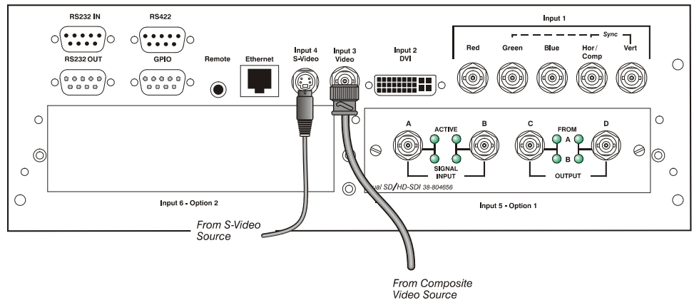
Figure 2.26. Connecting Composite Video
