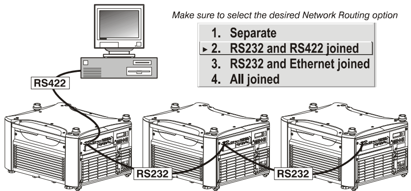
Figure 2.32. Mixed Serial Network
