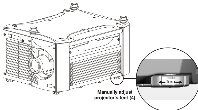
Figure 2.38. Adjusting the Feet Height
