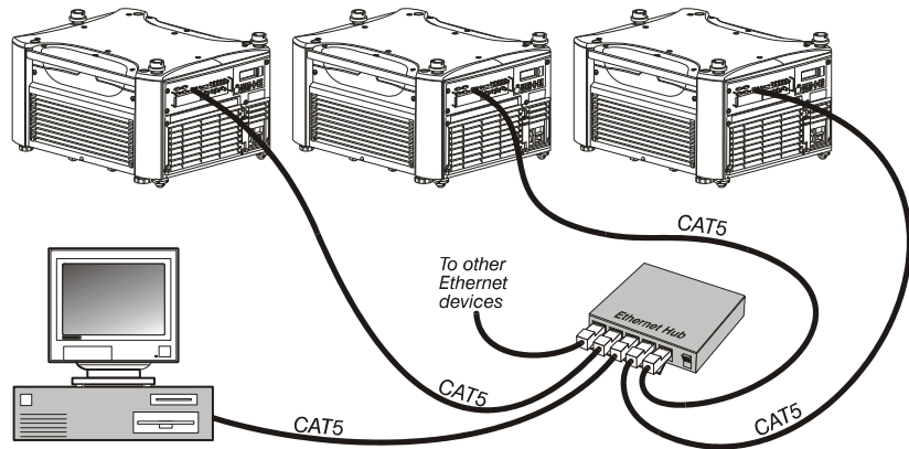
Figure 2.33. Typical Ethernet Network
