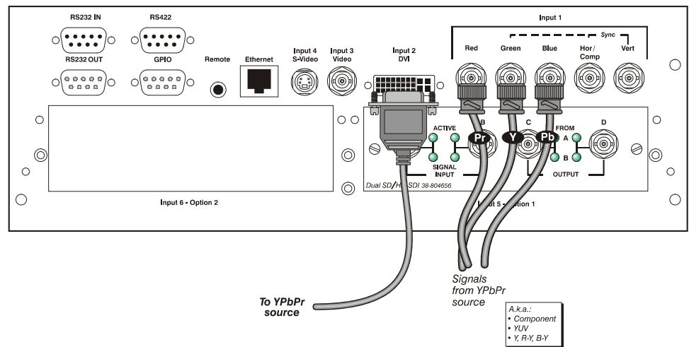
Figure 2.25. Connecting YPbPr
