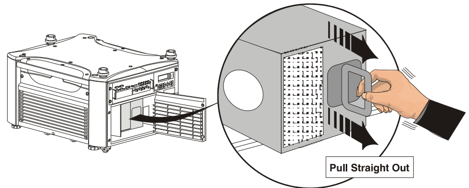
Figure 4.5. Remove Lamp Module
