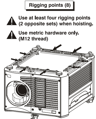
Figure 2.6. Bottom Rigging Points
