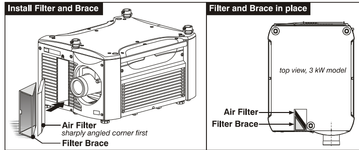
Figure 4.9. Installing the Angled Air Filter (3.0kW models only)
