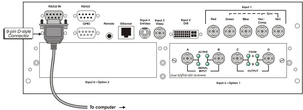
Figure 2.27. RS-232 Serial Communications
