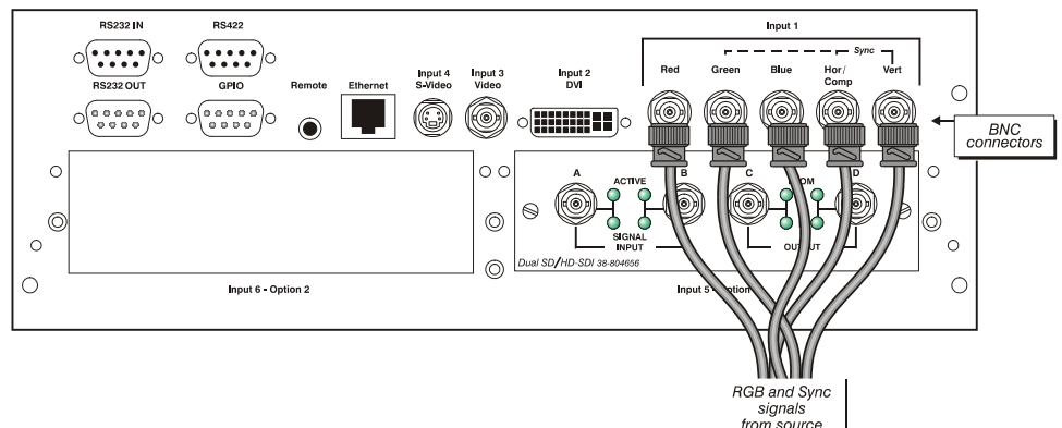
Figure 2.24. Connecting RGB Input
