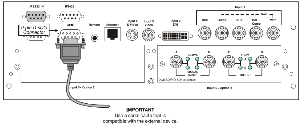
Figure 2.30. GPIO Port
