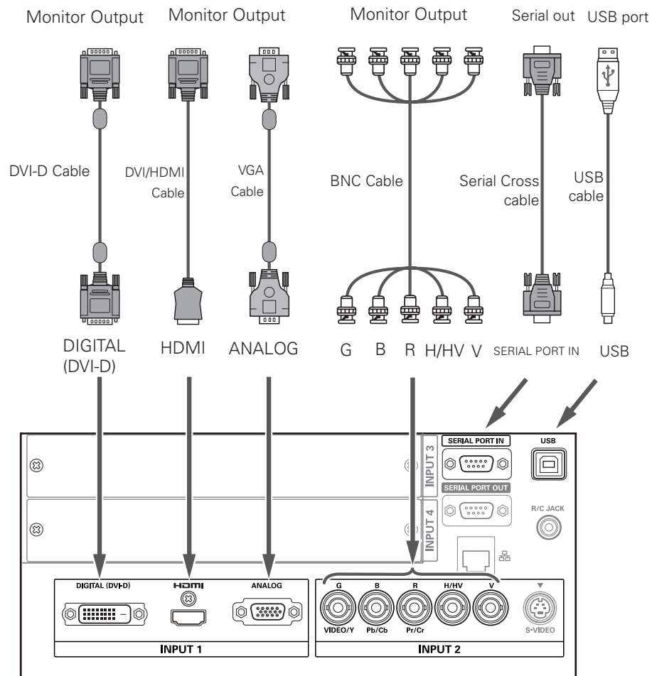
Terminals of the projector
