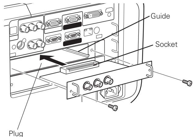
Figure shows Dual SDI Board
