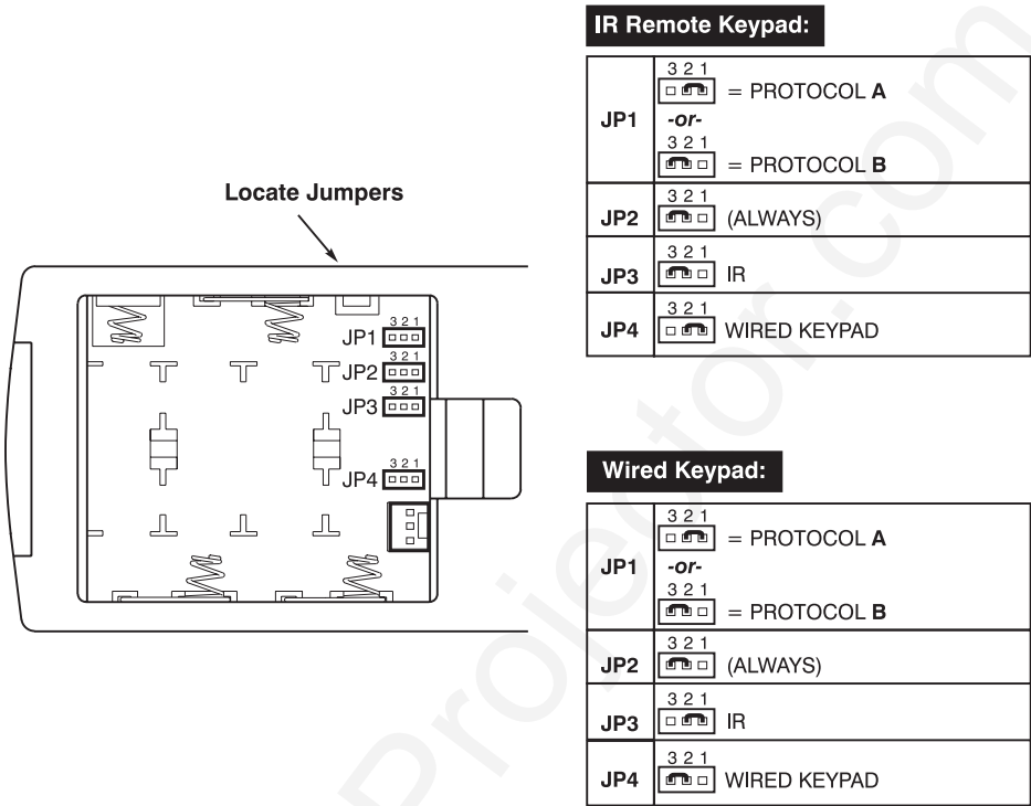
Figure 2.36. Locating and Setting the Jumpers
