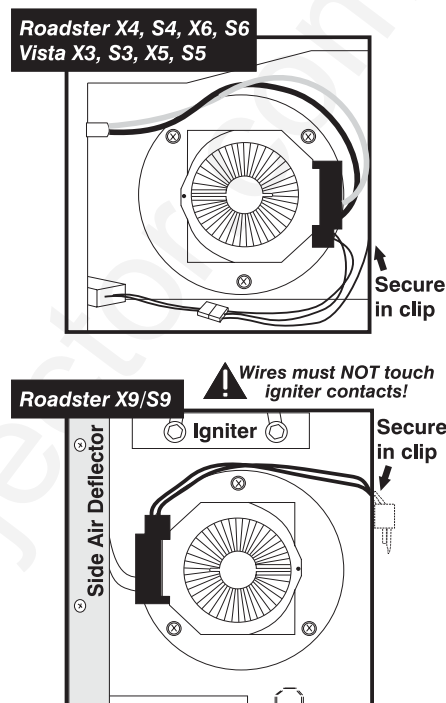
Figure 4.6. Lamp Orientation for Different Models
