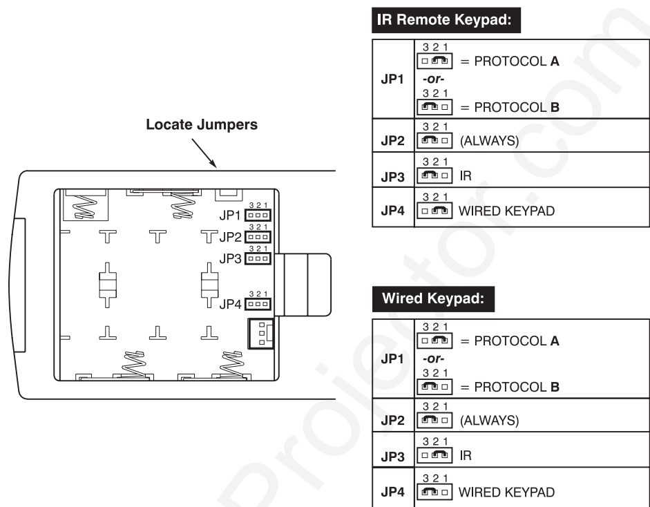
Figure 2.36. Locating and Setting the Jumpers
