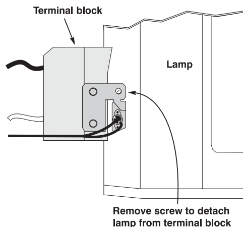
Figure 4.5. Detach lamp from terminal block (TOP VIEW)
