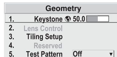
Figure 3.23. Geometry Menu
