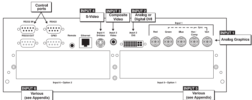
Figure 2.7. Input Panel
