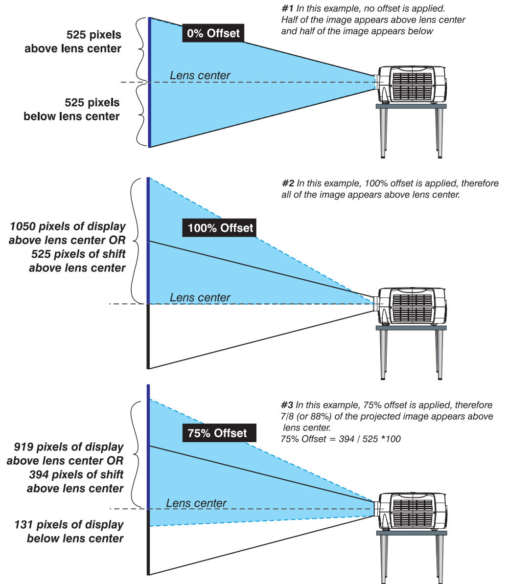
Figure 2.2. Vertical Offset Examples
