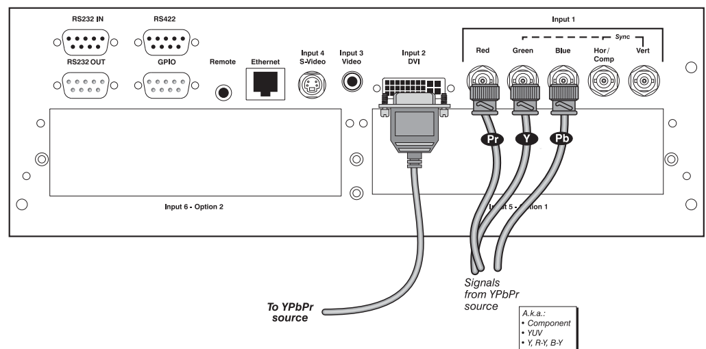
Figure 2.9. Connecting YPbPr sources
