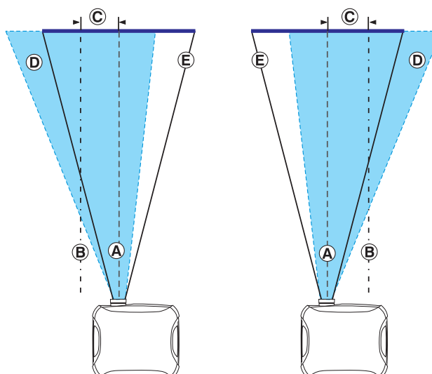
Figure 2.5. Lens Horizontal Offsets
