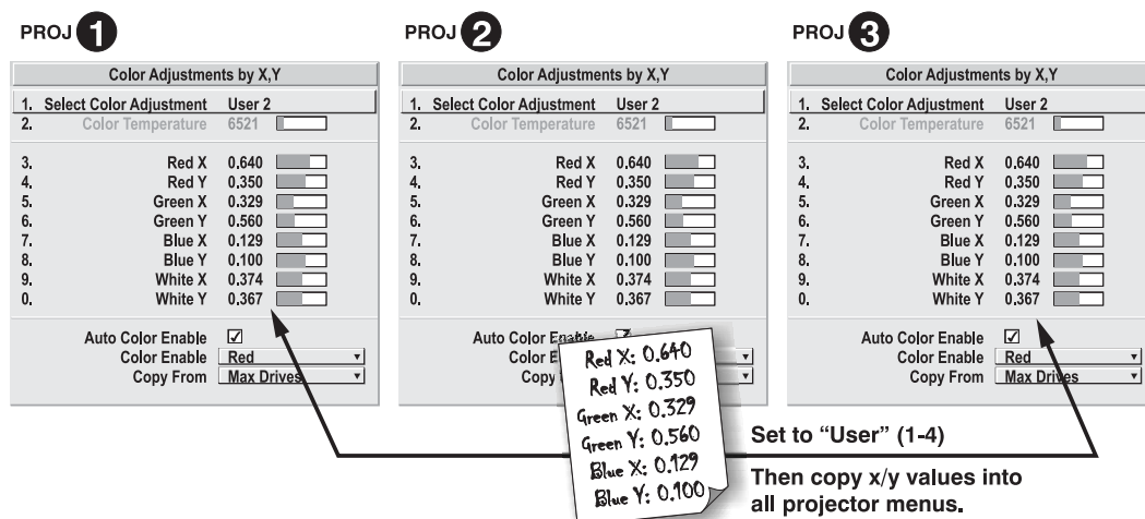
Figure 3.32. Copy X/Y Values into All Projectors
