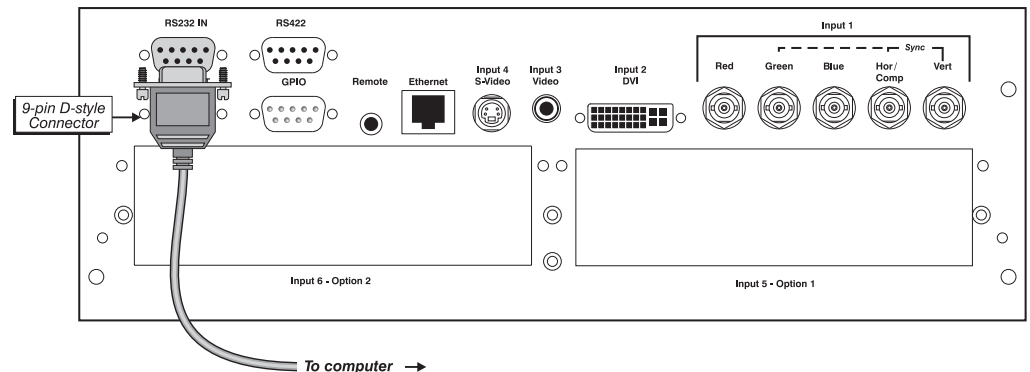
Figure 2.11. Connecting RS232
