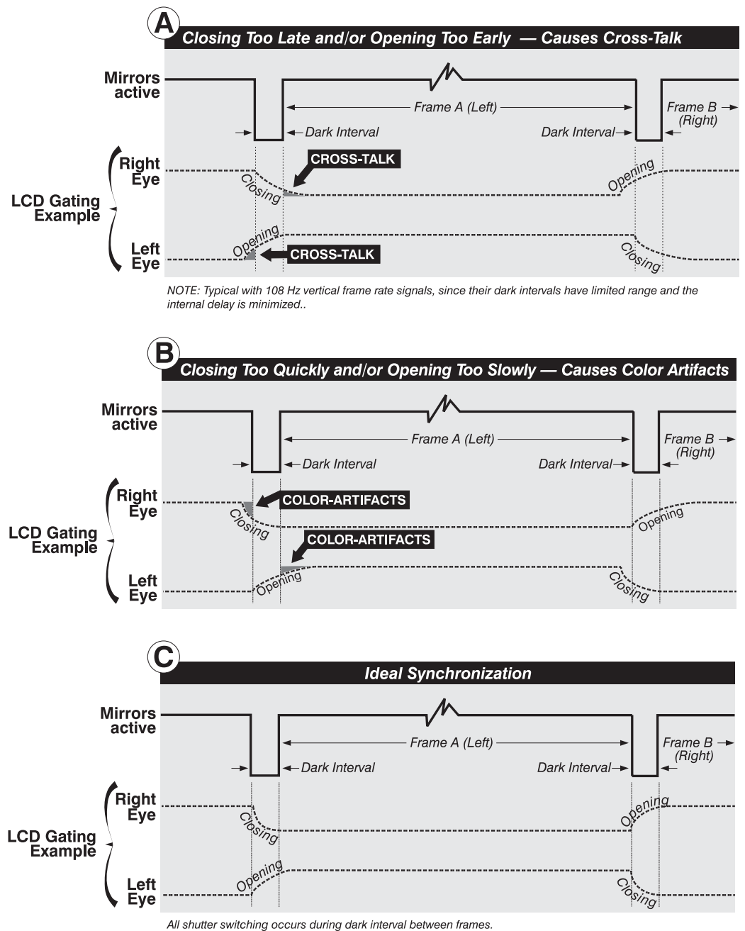
Figure 3.30. Examples of Poor and Ideal Synchronization
