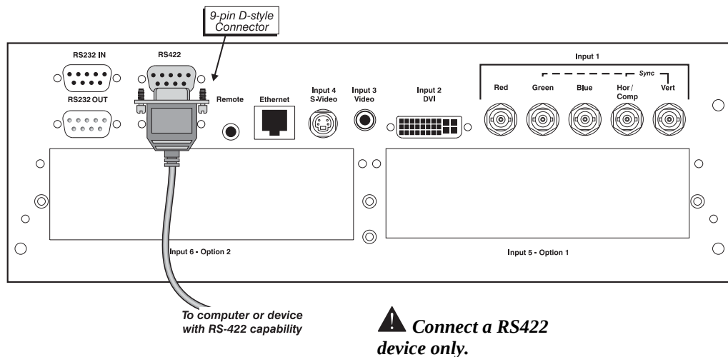
Figure 2.13. Connecting RS422
