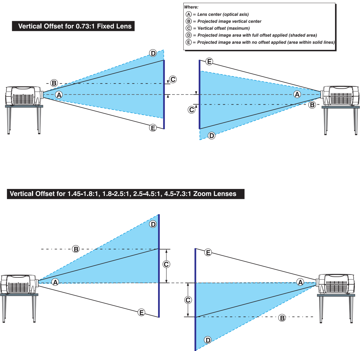
Figure 2.3. Lens Vertical Offsets
