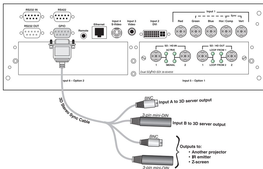
Figure 3.24. Connecting 3D Stereo Sync Cable
