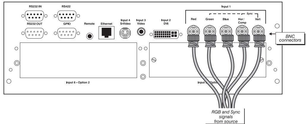
Figure 2.8. Connecting RGB and Sync
