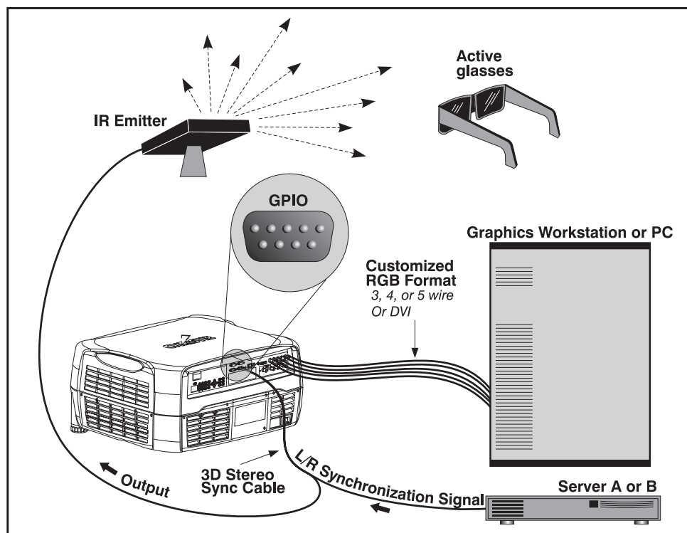
Figure 3.27. Typical 3D Configuration: Active Glasses & 3D Stereo Sync Cable
