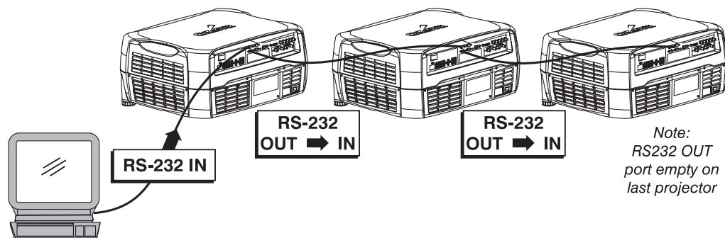
Figure 2.12. RS232 Network
