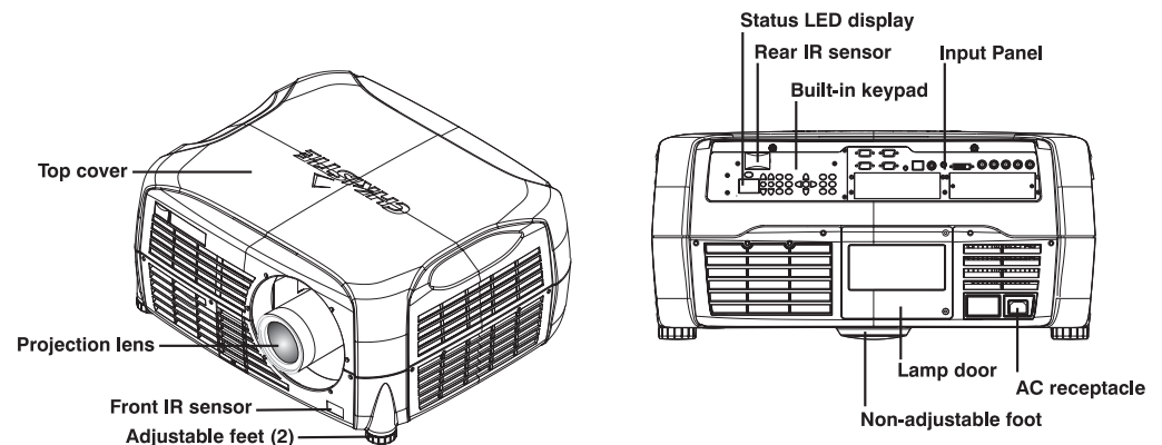
Figure 3.1. Projector Basics
