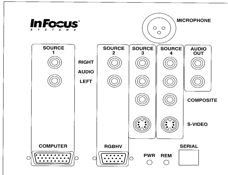
LitePro 550 side panel
