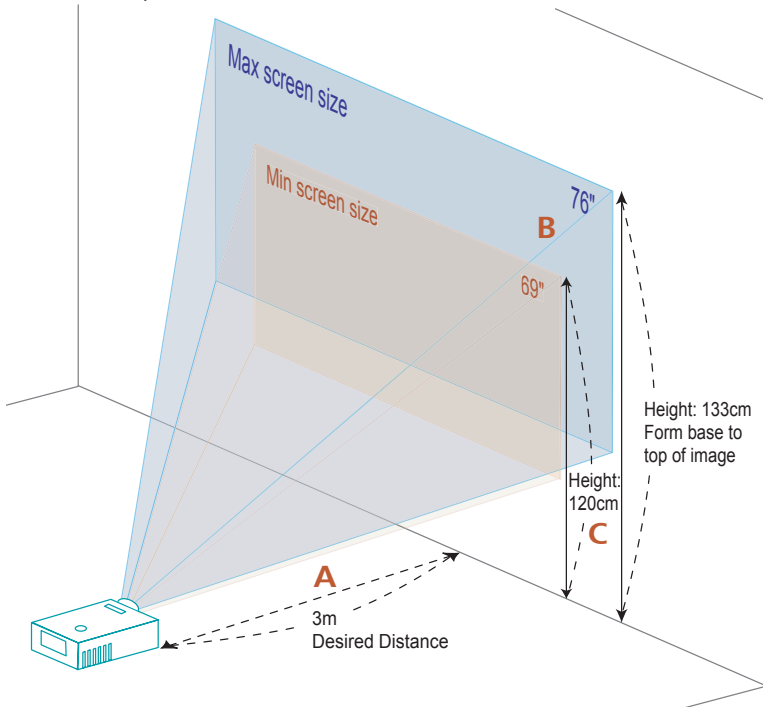
Figure: Fixed distance with different zoom and screen size. (only for X1260 series, X1160 series is Fixed zoom lens)
