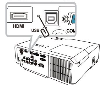
Shutdown switch
