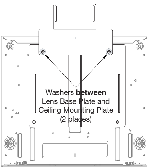
RS-900/CineWide or RS1100/CineWide with Prismatic Lens Base Plate and Ceiling Mounting Plate
