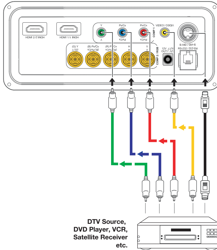
Figure 3-16. Composite, S-Video and Component Video Connections
