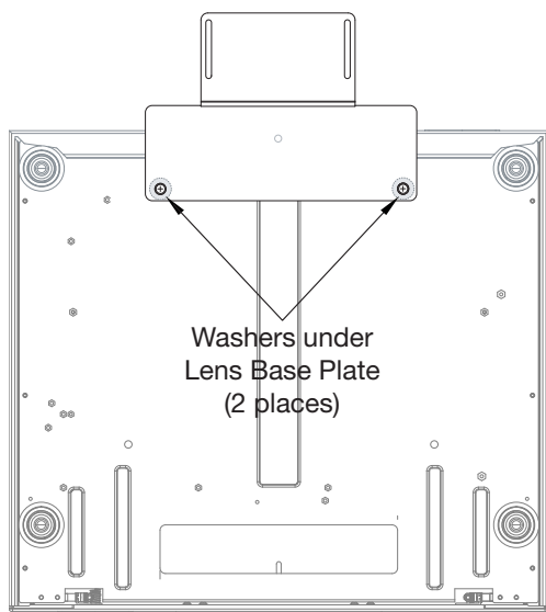
RS1100 Ultra/CineWide with Prismatic Lens Base Plate
