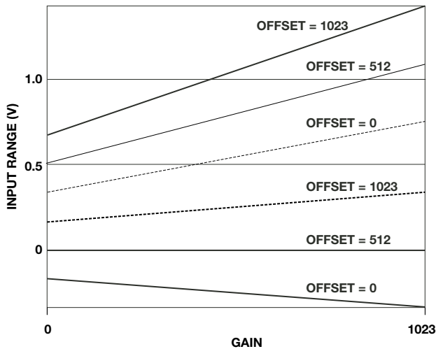
Figure 4-8. Gain and Offset
