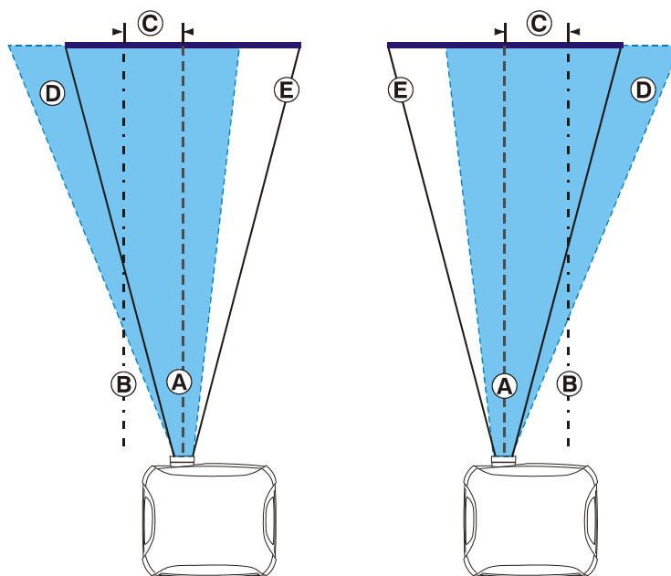
Figure 2.4. Lens Horizontal Offsets
